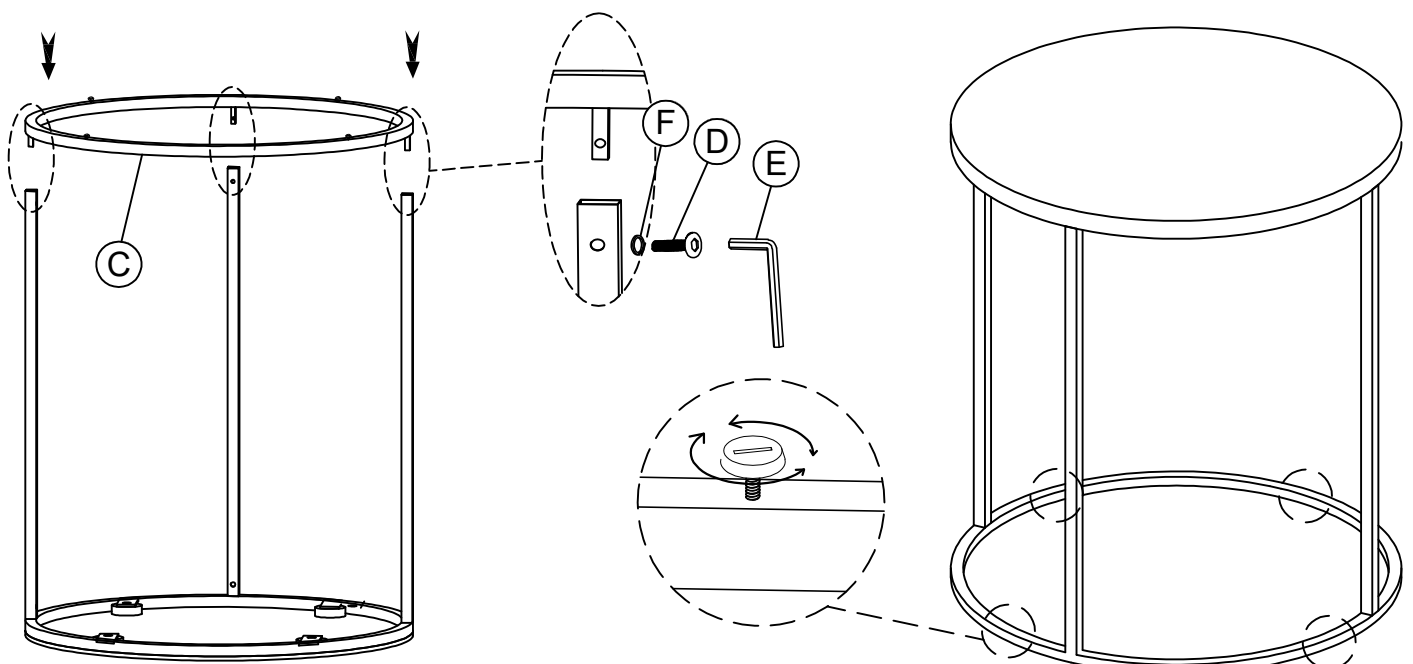
Adjustable Leveler
